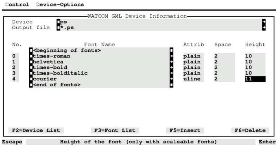
Figure 17. Define a new font
